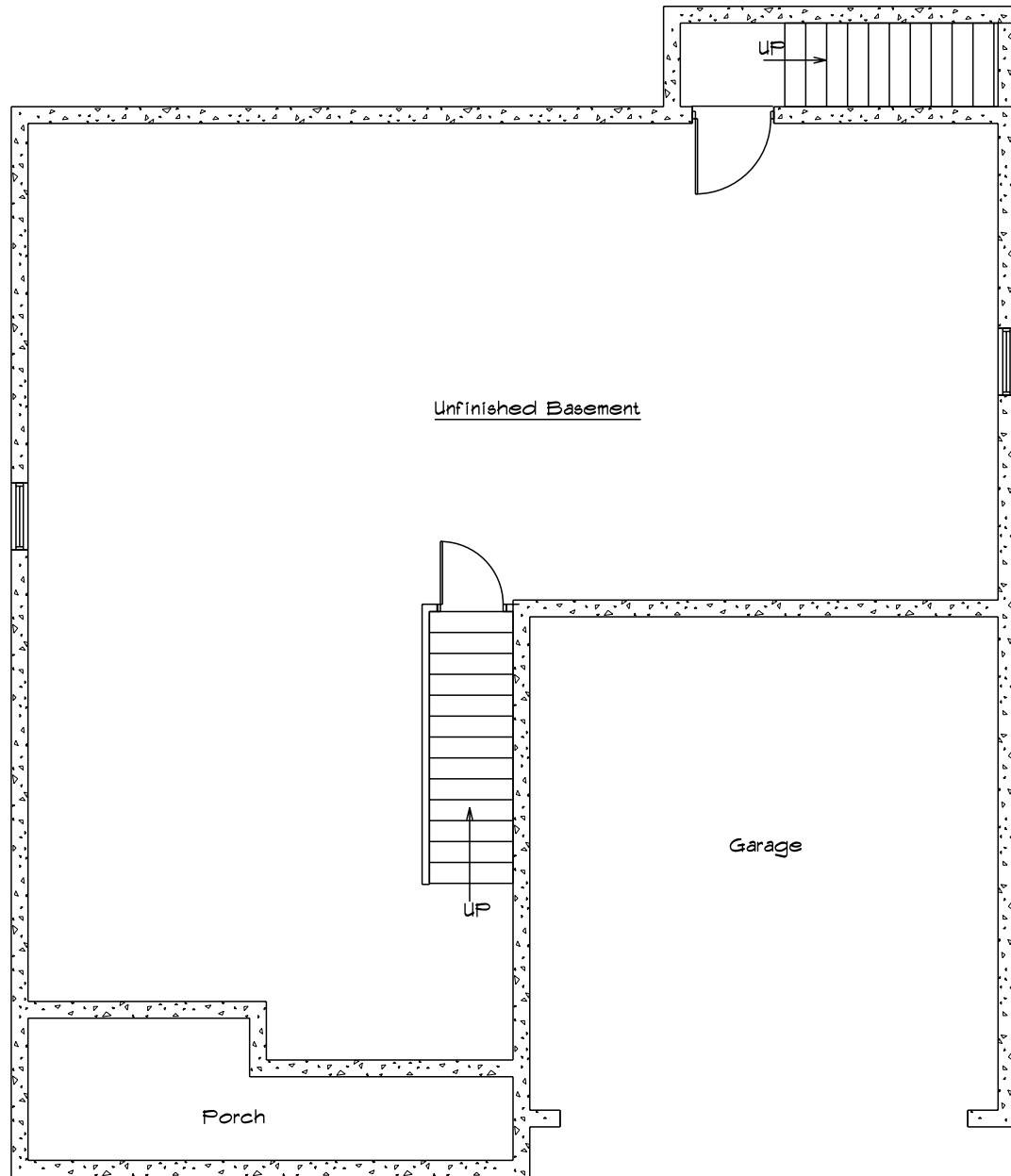
917 Willow Lane Basement Plan
